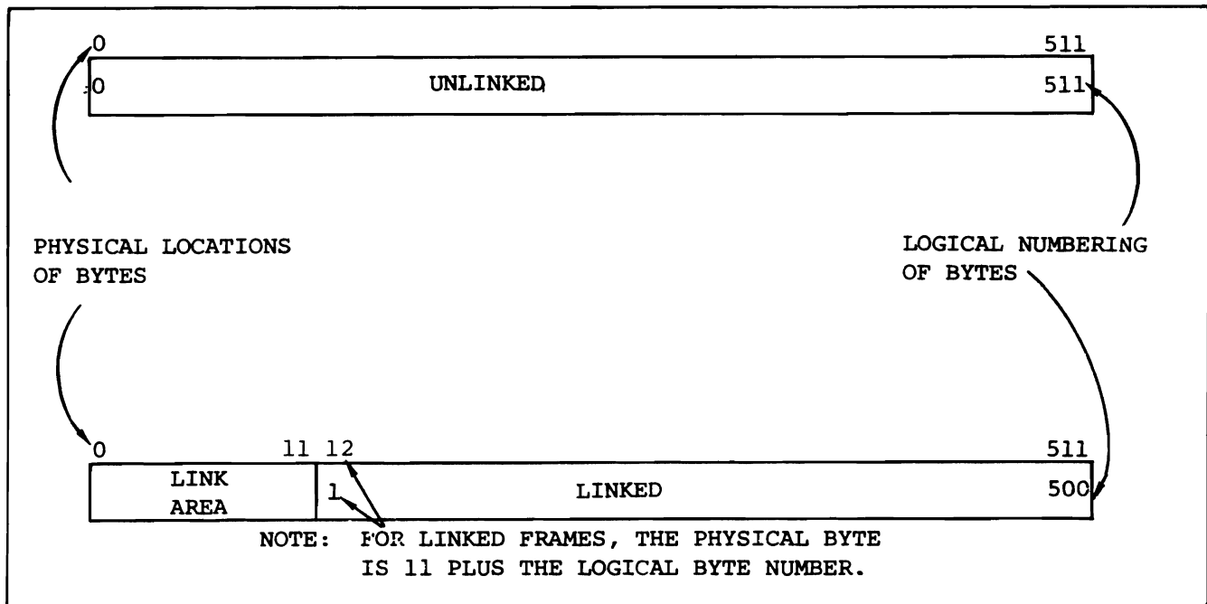
Figure 2-7. Unlinked Vs. Linked Frame Formats
