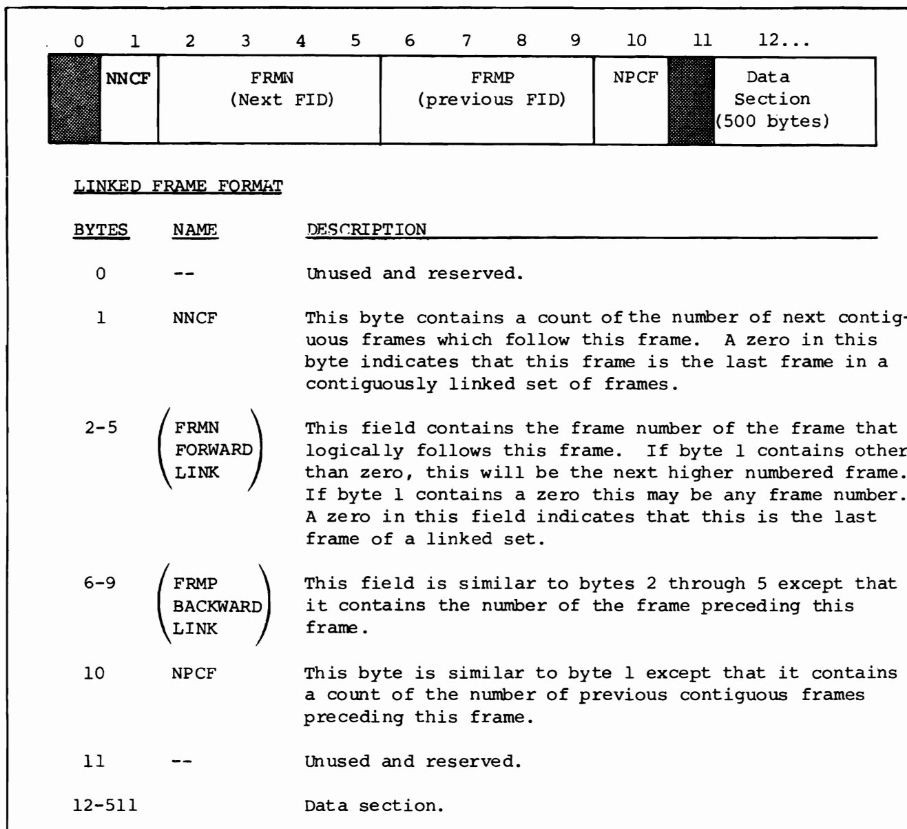
Figure 2-8. Linked Frame Format
