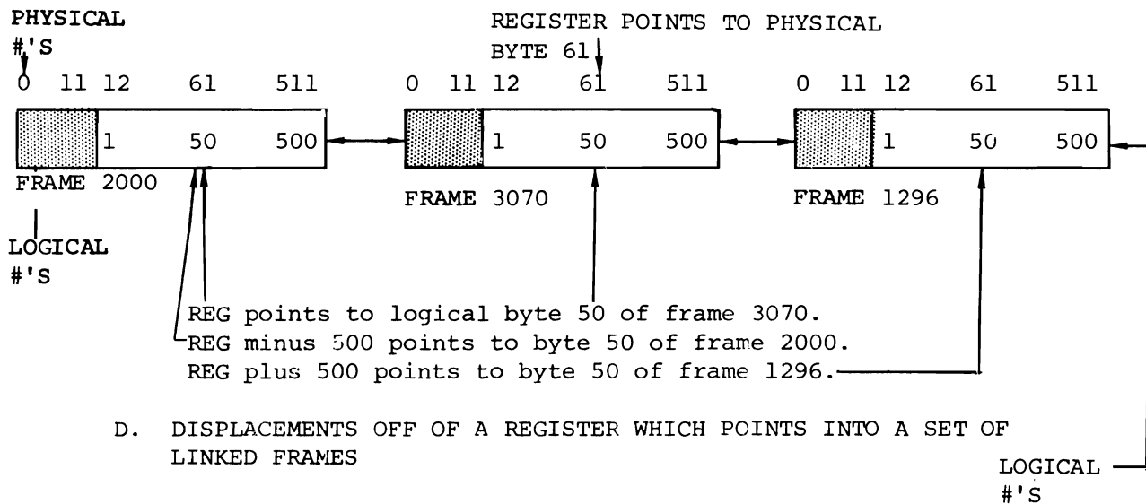
Figure 2-9. Examples of Linked Sets of Frames
