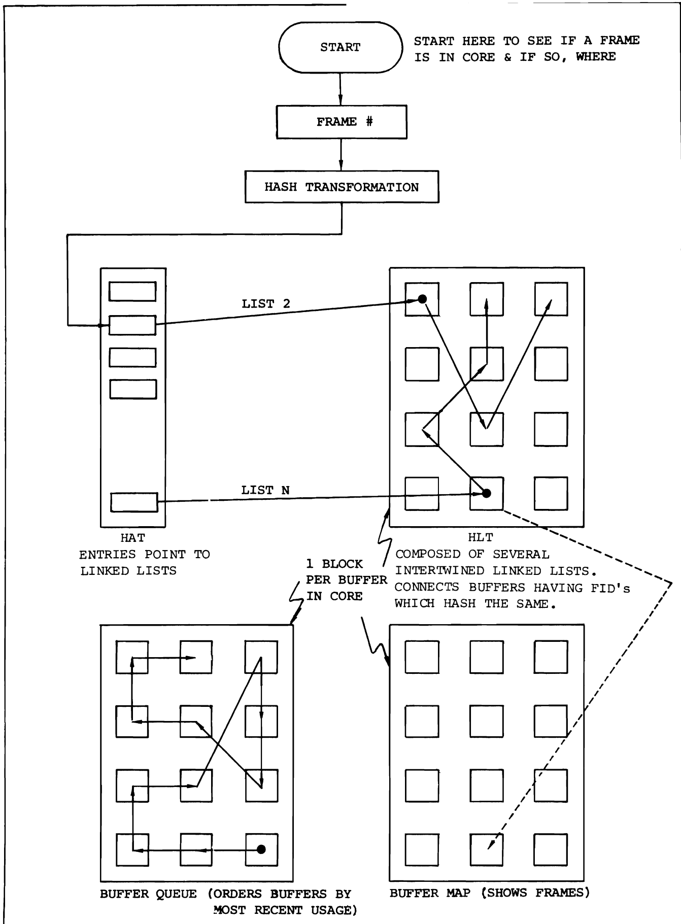
Figure 2-2. Memory Management Tables
