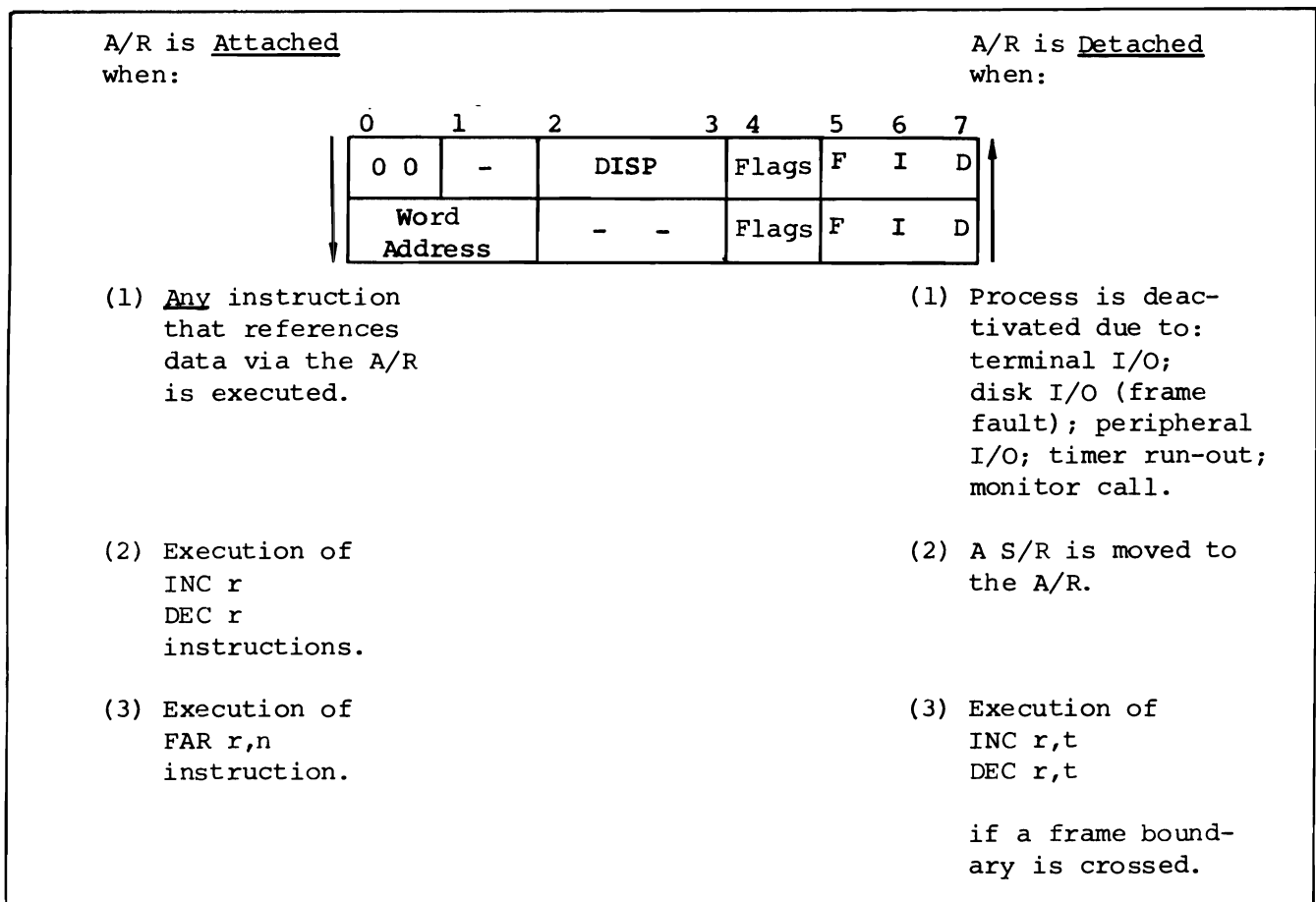
Figure 2-11. Attachment & Detachment of Address Registers
